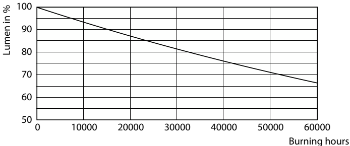
Lumen Maintenance Diagram - CorePro LEDtube HO 1200mm 18W865T8 AP
